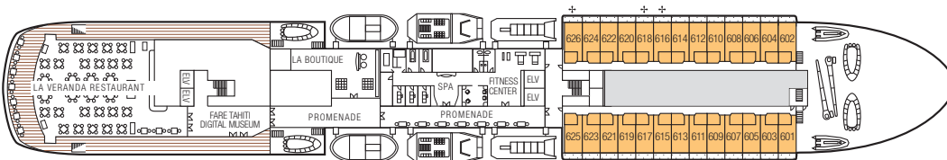
DECK SIX
